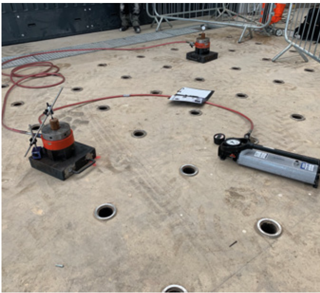
Macalloy 1030 Full Tensioning Unit
